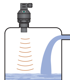
Level meter installation outside the influence of filling circulation
