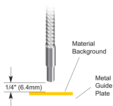
Fig. 1 Straight Position
