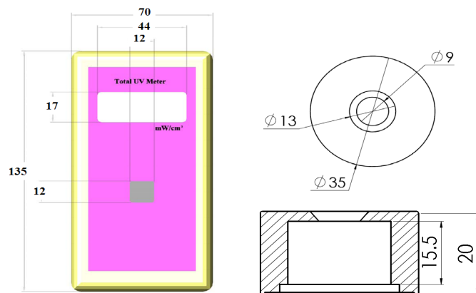
Fig2. Size of UV Radiometer7 and Sensor probe (Unit:mm)
