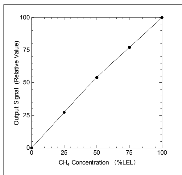
Fig 1 Sensitivity characteristic
