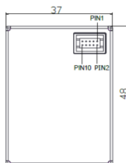
Figure 2 Connector Definition
